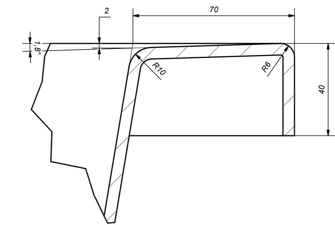
D (1:1)
